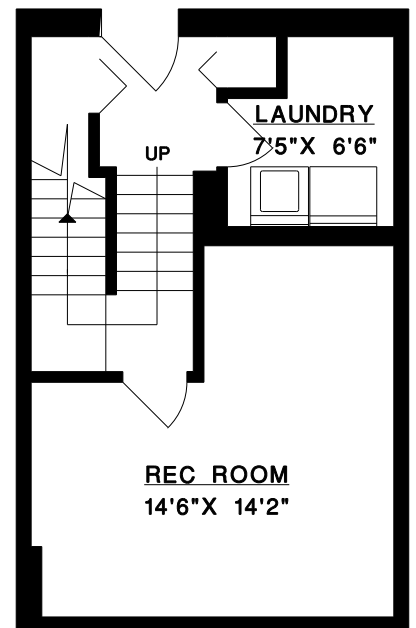
LOWER FLOOR
