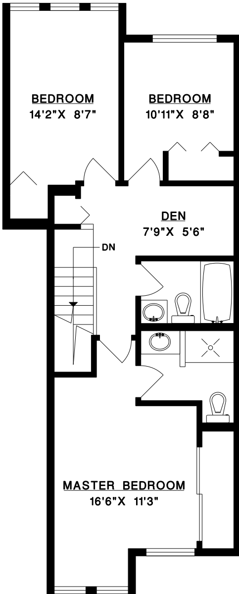
UPPER FLOOR
