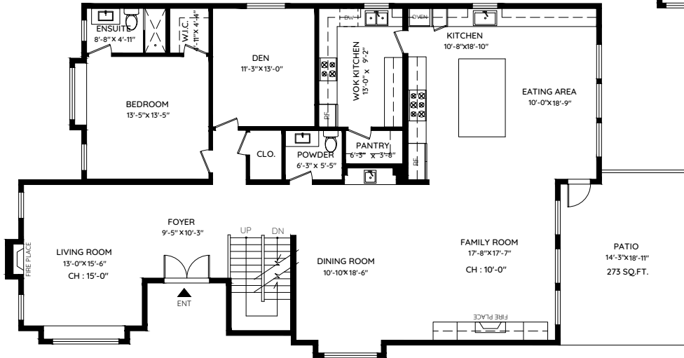
MAIN FLOOR 2,137 SQ.FT. CH: 10'-0"
