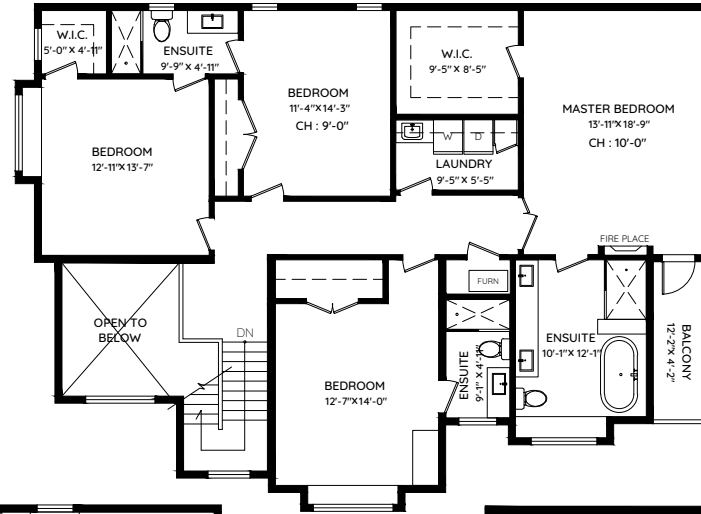
UPPER FLOOR 1,633 SQ.FT. CH: 9'-0"
